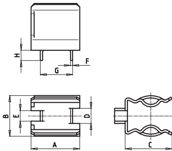
PINZE PER FUSIBILI 14x51 0900506 FUSE CLIPS FOR FUSES 14x51 0900506
