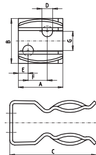
PINZE PER FUSIBILI 14x51 0900505 FUSE CLIPS FOR FUSES 14x51 0900505
